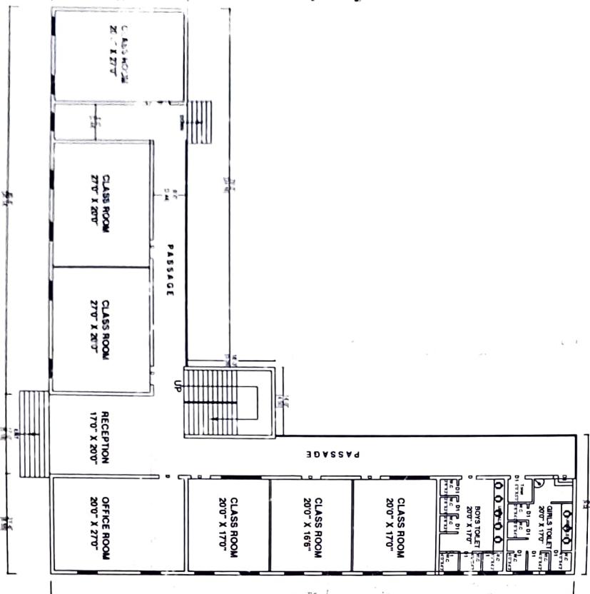
EXISTING GROUND FLOOR PLAN (BUILDING NO-1)
