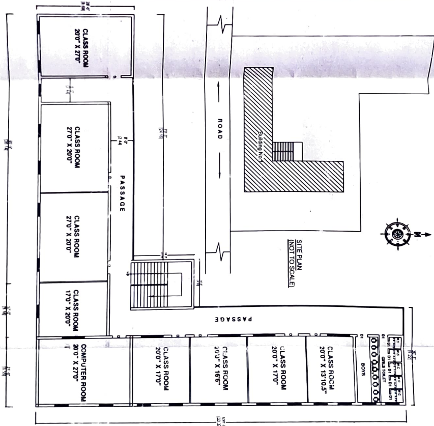
EXISTING FIRST FLOOR PLAN (BUILDING NO-1)
